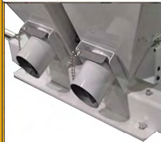
Standard Sightglass, Optional Drain Chute
