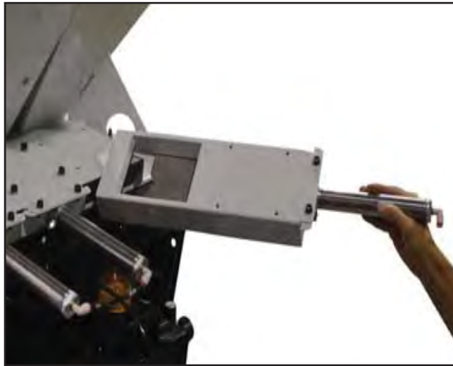
Cartridge-Style Metering Gate
